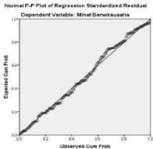
Gambar 2. Normal P-P Plot of Regretion Standardized Residual
